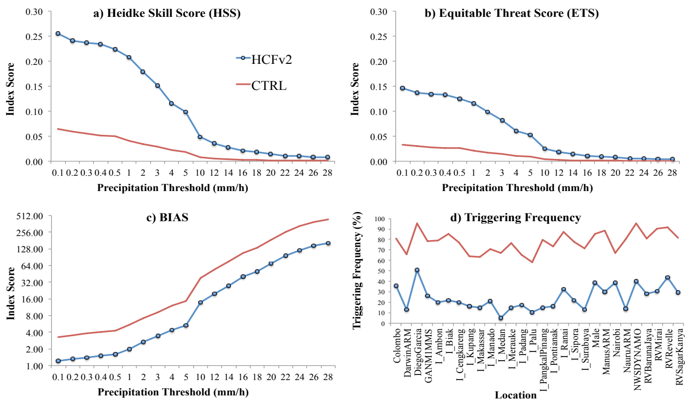
Figure 4: Comparison between the HCFv2 trigger and the original triggering (CTRL) mechanisms shown by (a) the Heidke Skill Score; (b) the Equitable Threat Score; (c) the Bias; and (d) the triggering frequency for each sounding release location.
